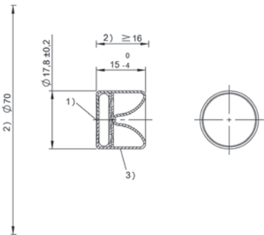
1) Sensing surface, 2) Clear zone, 3) Glass BIS00L8
