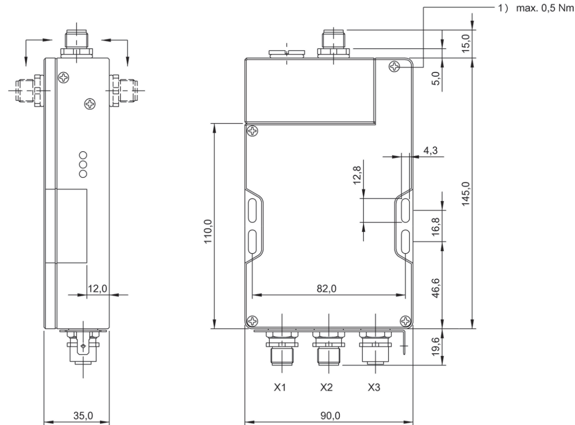
1) Tightening torque
