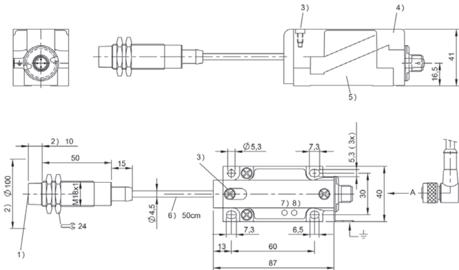
1) Sensing surface, 2) Clear zone, 3) Locking screw, 4) Module unit, 5) Mounting base, 6) Cable length, 7) Power, 8) Tag present
