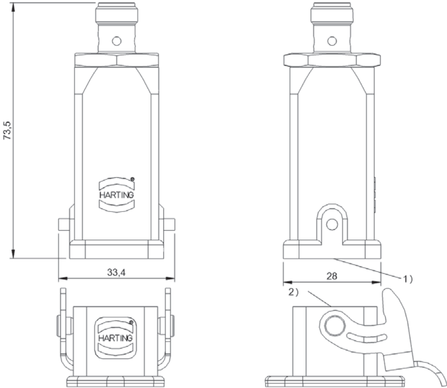
1) Sensing surface, 2) Data carrier
