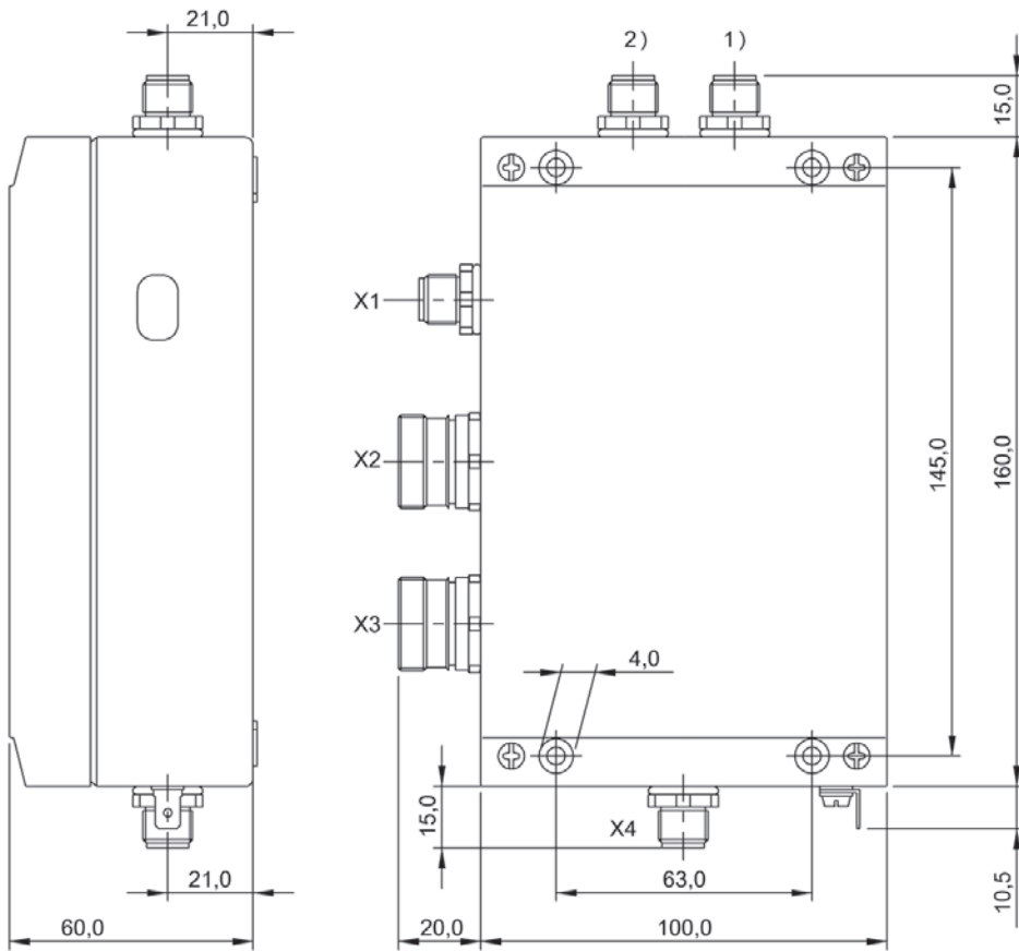
1) Head 1, 2) Head 2
