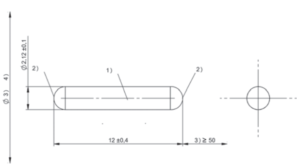
1) Sensing surface parallel, 2) Sensing surface axial, 3) Clear zone, 4) see corresponding R/W head BIS017F
