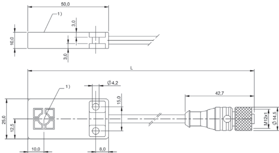
1) Sensing surface
