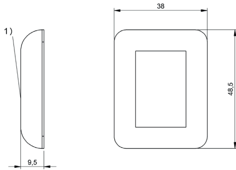
1) Sensing surface
