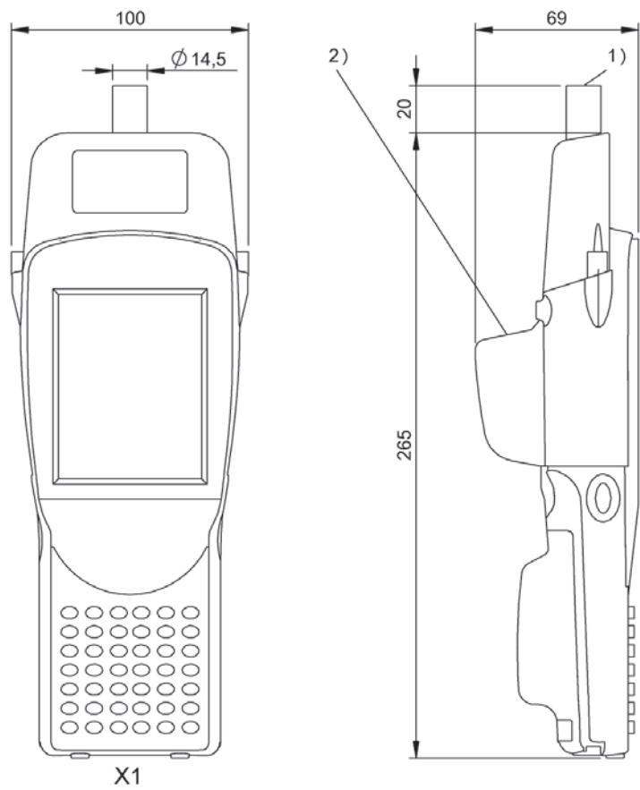
1) Sensing surface, 2) Barcode 2D-Scanner
